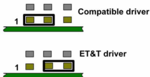
Pin description of J7 (Lower Layer)
