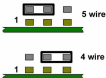
Pin description of J7 (Upper Layer)
